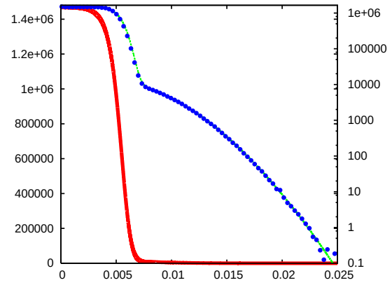
Figure 4: Beam density versus radius for a stationary, high-intensity bi-thermal distribution. The data are plotted on a linear scale (left axis, inner curve) and log scale (right axis, outer curve). The solid lines show the analytical solution as described in the text. The data points (circles, log scale) show the distribution after 10 focusing lengths, simulated using ML/I with 100 million particles. The halo is well-resolved out to a distance where the radial density is one million times smaller than the central density.
