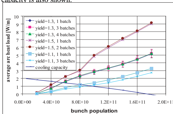
Figure 7: Simulated average arc heat load as a function of the bunch population for a bunch spacing of 25 ns at top energy (7 TeV), considering various values of \delta_{max} and computing the heat load over several numbers of consecutive 72-bunch trains. An estimate of the available cooling capacity is also shown.
