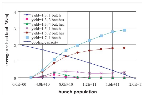
Figure 6: Simulated average arc heat load as a function of the bunch population for a bunch spacing of 25 ns at injection (450 GeV), considering various values of \delta_{max} and computing the heat load over several numbers of consecutive 72-bunch trains. An estimate of the available cooling capacity is also shown.
