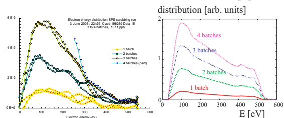
Figure 1: Electron energy spectrum for 1 to 4 batches. Left: energy spectrum measured with a variable bias voltage on the first day of the 2003 scrubbing run. Right: simulated full energy spectrum of incident electrons for \delta_{\max} = 1.4 , with a vertical momentum cutoff at 30 eV.
