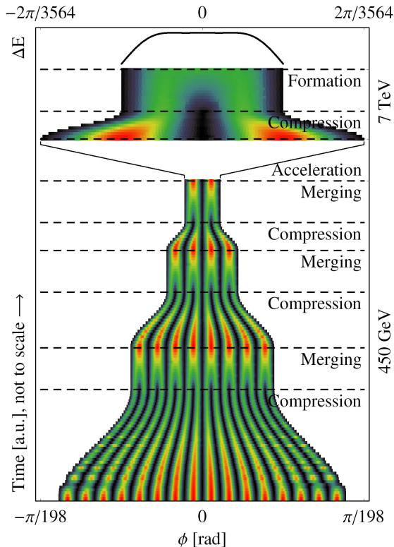
Figure 2: Mountain range plot of the separatrices (colour scale \propto \Delta E(\phi)^2 ) during formation of the long bunches.
