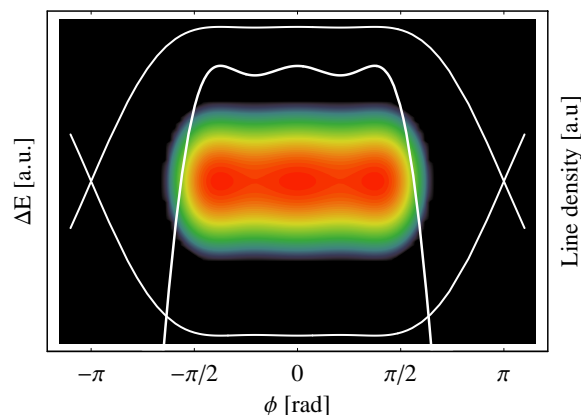
Figure 1: Longitudinal particle distribution and line density for a bunch kept in an optimized RF bucket generated by three harmonics. For h = 3564 , 2\pi corresponds to 7.5 m.
