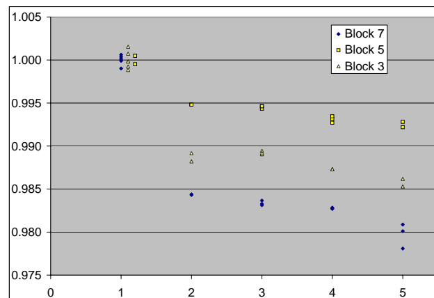
Figure 2: Magnetization loss versus radiation run number.
