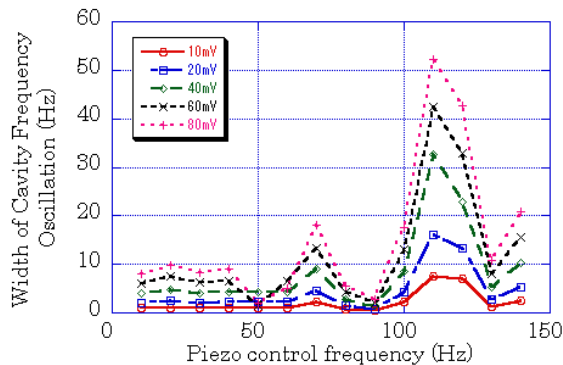
Fig.5 cavity frequency oscillation as a function of the frequency of the piezo control signal.
