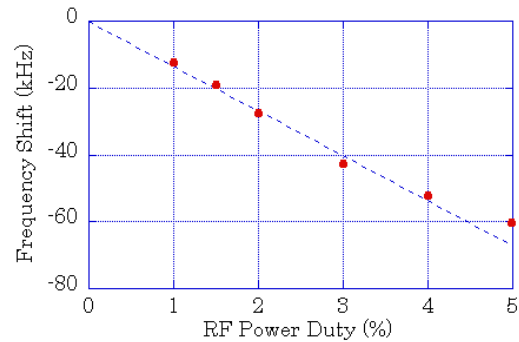
Fig.6 Measured frequency shift as a function of duty factor of the RF power.
