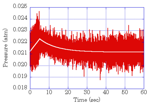
Fig.2 Pressure rise and decay in the cryostat for 5sec pulse operation.
