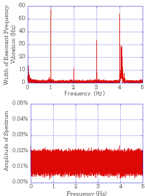
Fig.3 Spectrums of forward power (upper) and pickup power (lower) for high coupling and pulse mode.
