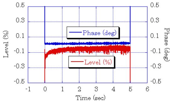
Fig.1 fluctuation of the accelerating field of the single-cell cavity in the long-pulse mode operation of 5 seconds with the new RF control system.
