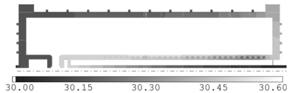
Fig.7 Calculated SHB temperature distribution of 3% duty.
