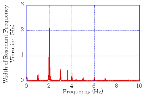
Fig.4 Spectrum of resonant frequency vibration for low coupling and CW mode.
