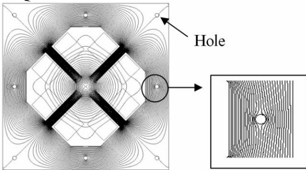
Figure 2: POISSON simulation.
