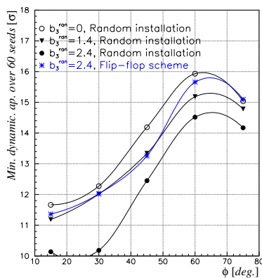
Figure 4: 100'000 turns LHC dynamic aperture [ \sigma ] at injection as a function of the phase space angle \phi = \arctan(A_x/A_y) .
