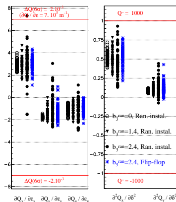
Figure 5: Anharmonicity coefficients \partial Q_{x,y}/\partial \epsilon_{x,y} [ 10^3 \text{ m}^{-1} ] and second order chromaticity Q''_{x,y} [ 10^3 ] due to a_3 , b_3 and b_4 in MQ's and MB's at injection. Statistics performed over 60 seeds.
