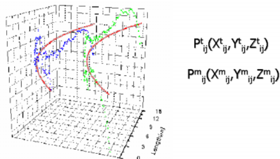
Figure 1: Mechanical axis of a two-in-one LHC dipole and best fit in 3D with the geometrical axis (courtesy of M. Bajko).
