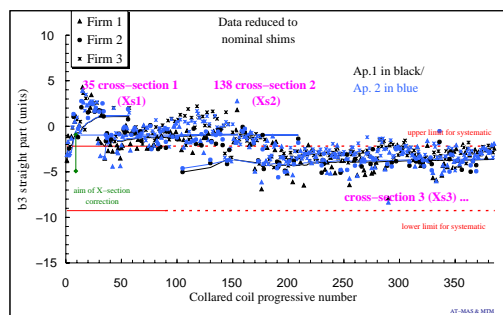
Figure 3: Evolution of the b_3 harmonics in the collared coils of LHC dipoles (courtesy of E. Todesco).
