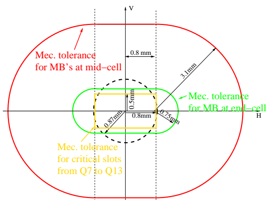
Figure 2: Mechanical tolerances for the dipole extremities (dashed line) and the magnet body (solid lines).
