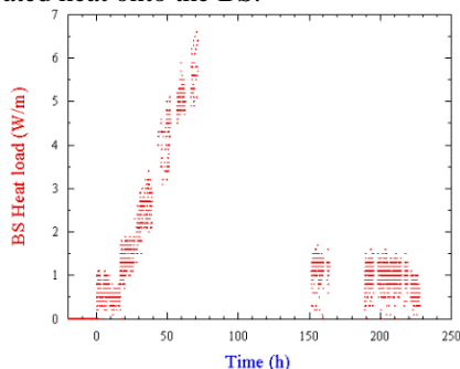
Figure 1: Heat load due to condensed gases onto the BS when 2 batches circulated through COLDEX.
