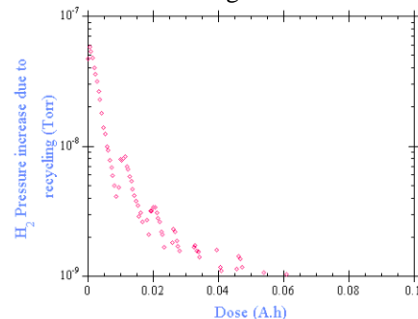
Figure 2: H_2 dynamic recycling pressure when 2 batches circulated with 10^{15} H_2/cm^2 condensed onto the BS
