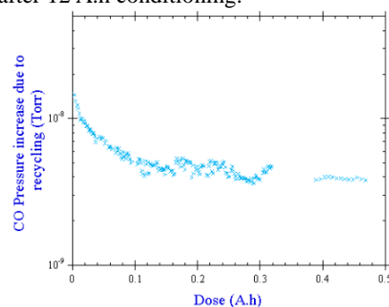
Figure 3: CO dynamic recycling pressure when 1 batch circulated with 5 \cdot 10^{15} CO/cm^2 condensed onto the BS.
