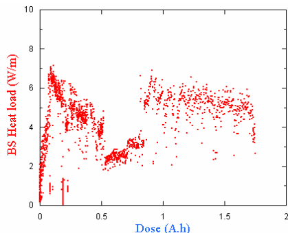
Figure 4: BS heat load when 1 to 4 batches circulated with 60 \cdot 10^{15} CO/cm 2 condensed onto the BS.
