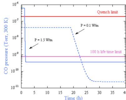
Figure 5: Vacuum transients computed after a quench and the condensation of 25 \cdot 10^{15} CO/cm 2 onto the BS.
