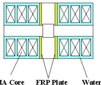
Fig. 1. Schematic of direct water cooling.
