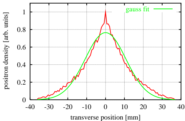
Figure 6: Beam profile behind the capture optics.
