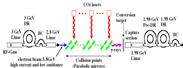
Figure 10: Proposed layout for the polarized positron source for GLC.
