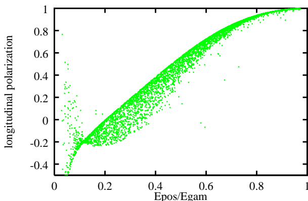
Figure 7: Longitudinal polarization of positrons produced by pair production as function of the fractional energy. The incoming photon is fully circular polarized.
