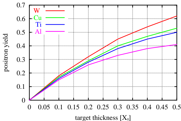
Figure 3: Positron yield for different materials as function of the target thickness. The incoming photon beam was in this example generated by a 250 GeV electron passing through a 1 m long wiggler of 1.7 T field strength.
