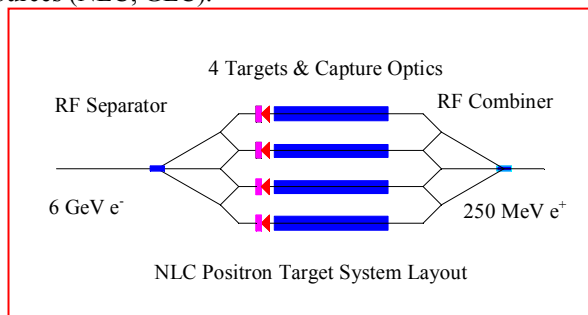
Figure 1: The NLC positron source with RF separators and combiners. 3 targets are used during normal operation; the fourth is a spare target.
