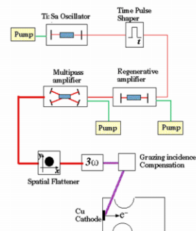
Figure 1: Conceptual layout of SPARC laser system.
