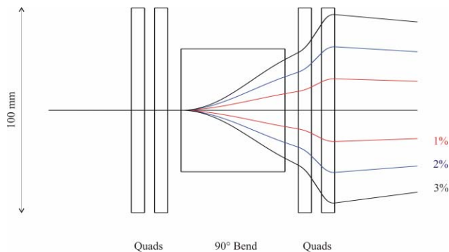
Figure 5: |\Delta q|/q=1\% \dots 3\% separation in the cryogenic storage ring as calculated with COSY infinity.
