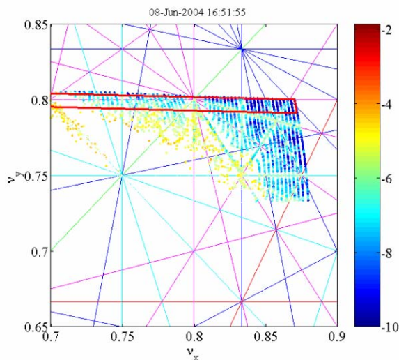
Figure 5: Frequency map of TME lattice.
