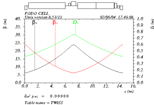
Figure 1: Existing 72° FODO cell with 3.2° deflection per cell.
