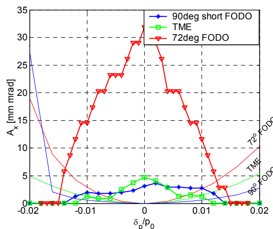
Figure 8: Off-momentum apertures for the different lattice types 72° FODO, TME, and 90° short FODO. Tracking has been performed with an aperture limitation corresponding to the real physical aperture of approx. 30 mm mrad.
