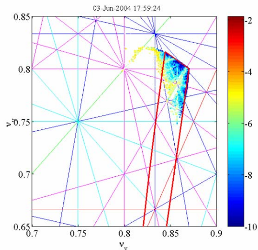
Figure 4: Frequency map of short 90° FODO lattice.
