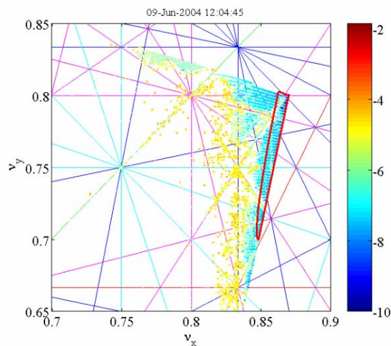
Figure 6: Frequency map of 72° FODO lattice and damping wigglers. Thick red line encompasses the area in tune space corresponding to the physical aperture.
