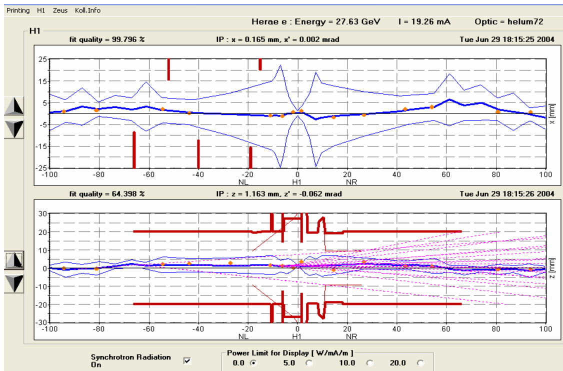
Figure 1 Online display of the positron orbit near the H1 detector in HERA. The lines are the best fit orbit with its 10 sigma envelope and the dots the values from the BPMs. Drawn in the lower half are the vertical chamber dimensions including absorbers and the positions of the movable collimators as well as the direction of the synchrotron radiation fans (dashed lines).
