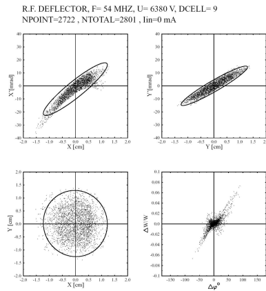
Figure 9: Emittances 11 cm behind the 9 cell deflector.
