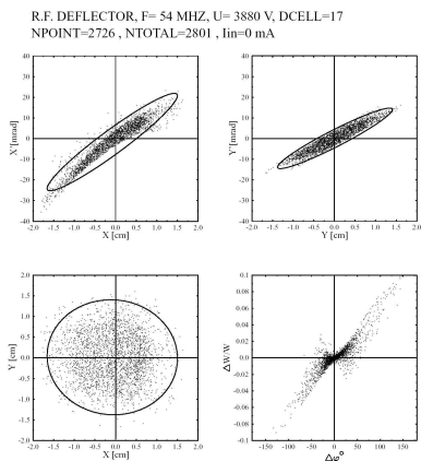
Figure 8: Emittances 11 cm behind the 17 cell deflector.
