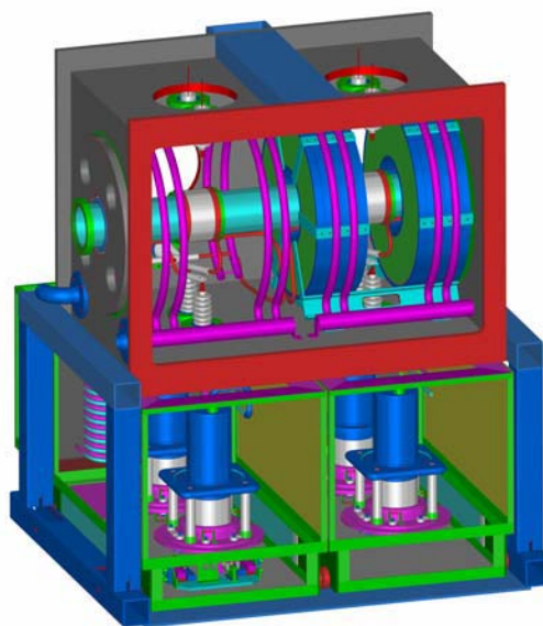
Fig. 2: Two cavities are combined in one box. The rf power stage is located directly below the cavity box.
