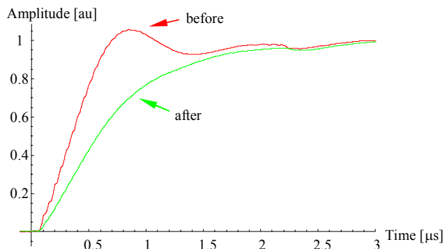
Figure 2: Measured MKQH kicker pulse characteristics
