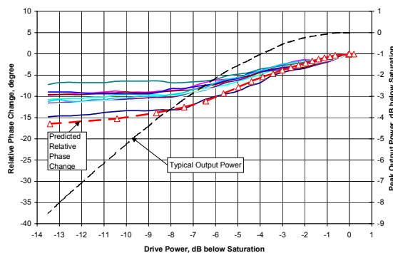
Figure 5: Relative Phase Change vs. Drive Power
