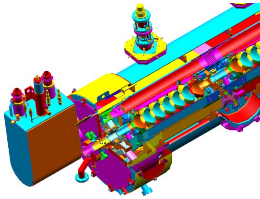
Figure 1: Cryomodule design.
