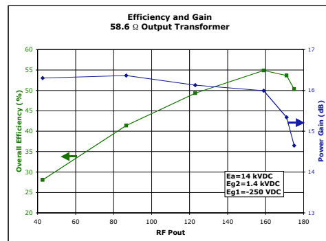
Figures 2a (top) and 2b (bottom): IPA Test
