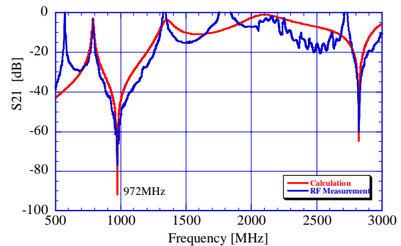
Figure 7: Frequency characteristic of a HOM coupler.
