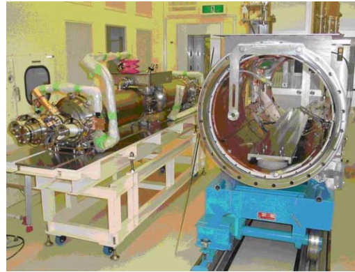
Figure 1: Assembling of the prototype cryomodule.
