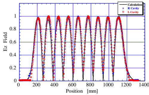
Figure 3: Field distribution after pre-tuning.
