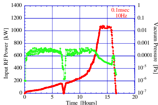
Figure 5: RF processing in the initial test.
