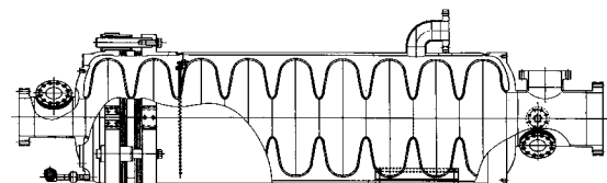
Figure 2: A 972MHz 9-cell cavity of \beta=0.725 , (L cavity).
