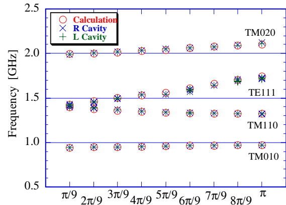
Figure 9: Frequency distribution of HOMs.
