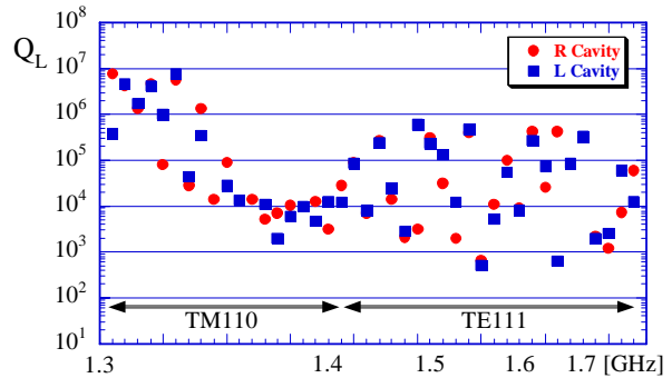
Figure 10: Measured Q_L of TM110 and TE111 modes.
