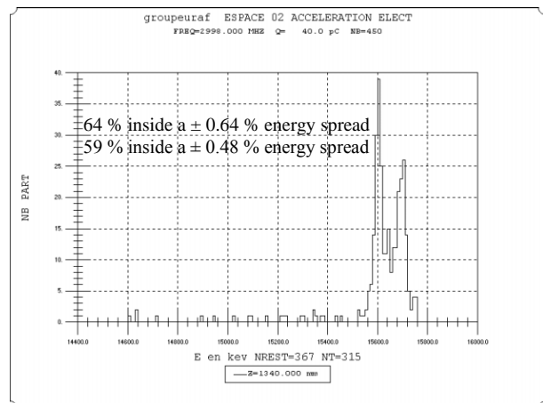
Figure 2 : Energy histogram at the buncher exit for the 120 mA mode.
