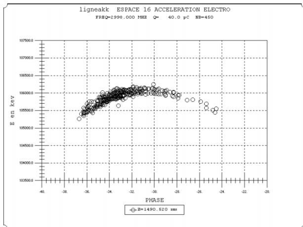
Figure 3 : Phase-energy diagram at the linac exit for the 120 mA mode.
