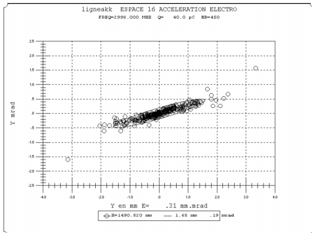
Figure 4 : Emittance at the linac end for the 120 mA mode.
