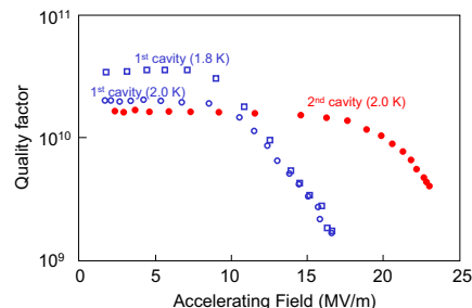
Figure 5: Vertical cavity tests of the HOBiCAT cavities at DESY.
