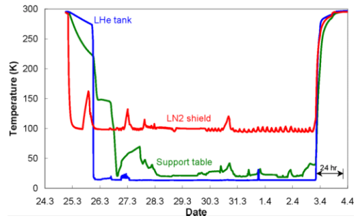
Figure 3: Temperatures of the LN 2 shield, the support table and the dummy helium tank during HOBICAT commissioning. Measurements were made with CLTS sensors which were not fully calibrated at LHe temperatures and therefore bottom out at around 10 K.
