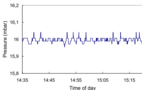
Figure 4: Helium bath pressure in the helium tank used for HOBiCAT commissioning. The dynamic load at this time was of order 20 W.
