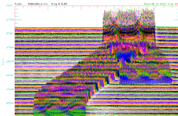
Fig.3: Slip-stacking of 6\text{e}12 protons in Main Injector
