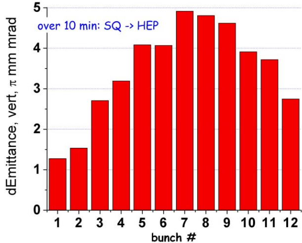
Fig.7: Emittance growth along pbar bunch train
