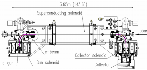
Figure 5: The first Tevatron Electron Lens.
