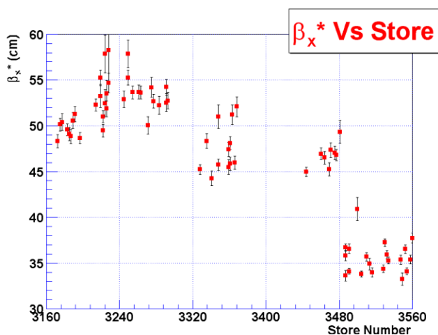
Fig.4: \beta_x^* as fit parameter of D0 luminous region analysis in stores from Jan., 13 to June 5, 2004, courtesy of J.Estrada, A.Chandra (D0 collaboration)
