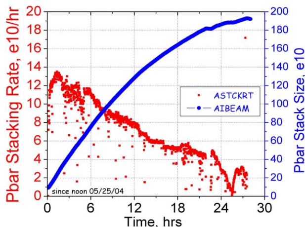
Fig.2: Typical cycle of Antiproton Accumulator operation antiprotons to the Recycler at the rate of 40\text{e}10/\text{hr} .
