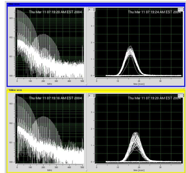
Figure 3: Spectra and profiles before rebucketing showing the effect of the Landau cavities.
