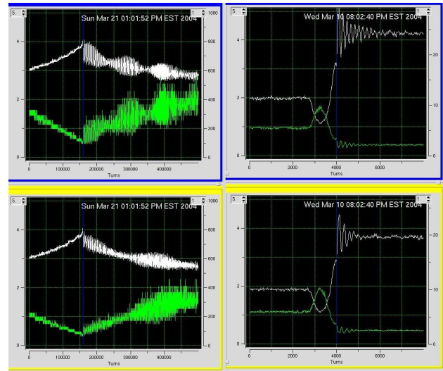
Figure 2: Bunch width (Green) and amplitude (White) in both rings during transition, and rebucketing.
