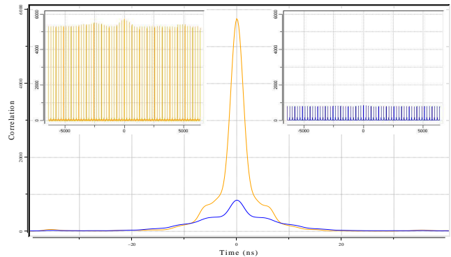
Figure 6: Correlation along the ring with 56 bunches injected, and the vertex for interaction region IR 2, after rebucketing at the start of store 4829 (Orange), and after 7 hours (Blue). The ratio between IR's can substantially deviate from the expected 52/56 ratio due to non-uniform filling of the rings.
