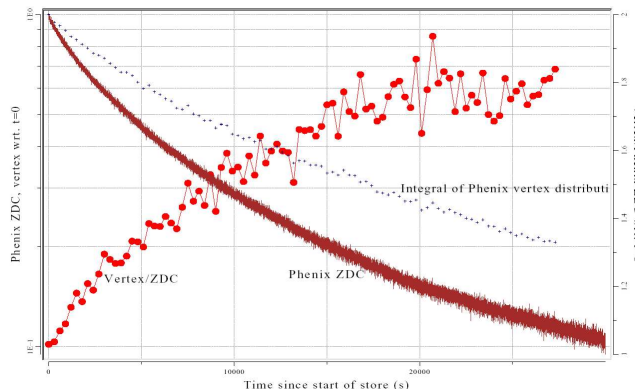
Figure 8: Phenix ZDC rates (Brown), and integral of vertex (Blue) normalized wrt. the start of store 4829, and deduced emittance increase (Red) as a function of time in store.
