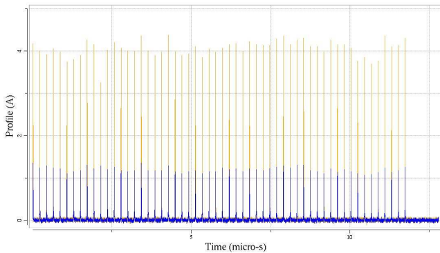
Figure 5: Longitudinal profiles along the Blue run after rebucketing (Orange), and at the end of store (Blue), showing a typical 56 bunch fill pattern and the abort gap.
