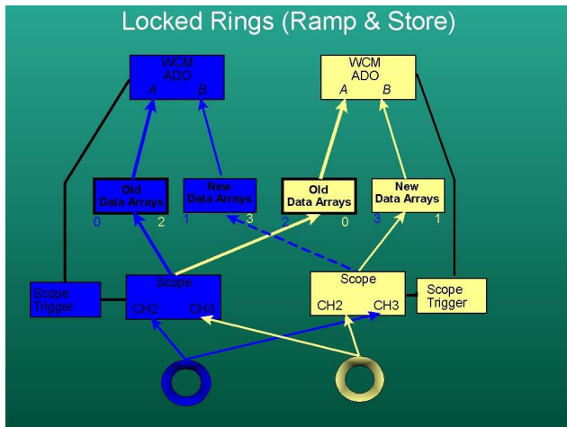
Figure 1: Blue and yellow wcm signal connections
