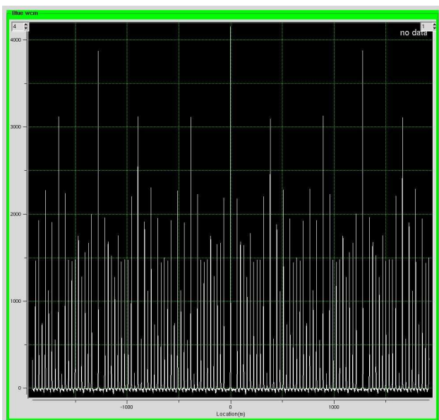
Figure 7: Vertex distribution for an irregular 45 bunch pattern. Horizontal scale is in meters. Peaks are at 0 m and at \pm 1/3 of the circumference of RHIC = \pm 1278 m.
