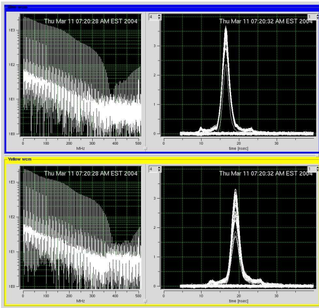
Figure 4: Spectra and profiles after rebucketing.
