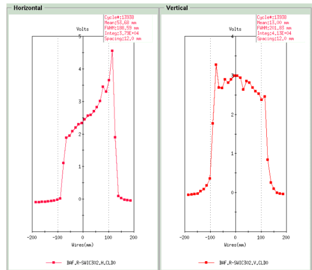
Figure 6: Beam misalignments at the entrance of the horizontal (O1) or Vertical (O2) octupoles affect the uniform beam distribution at the target. A horizontal corrector magnets can be used to correct such beam misalignments.
