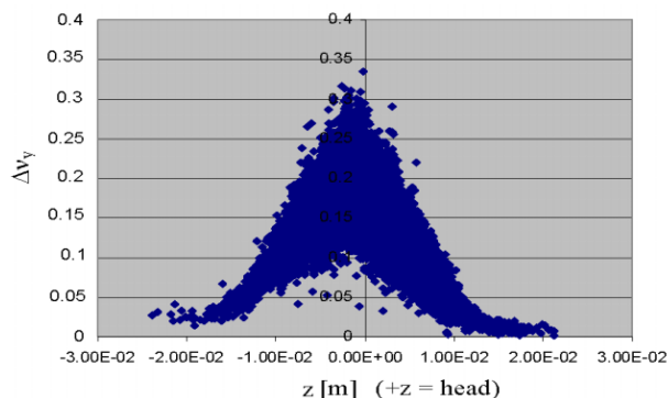
Figure 4: Vertical tune shift after passing through the TESLA wiggler beam line which has 432 meters of wiggler in 520 meters of beam line. An electron cloud density of 6 \text{e} 12 \text{ e m}^{-3} is assumed. No magnetic field was included.
