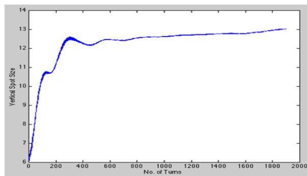
Figure 3: Simulation of single-bunch instability from electron cloud in the TESLA DR using QUICKPIC code, for a cloud density of 1 \text{e} 10 \text{ e m}^{-3} .
