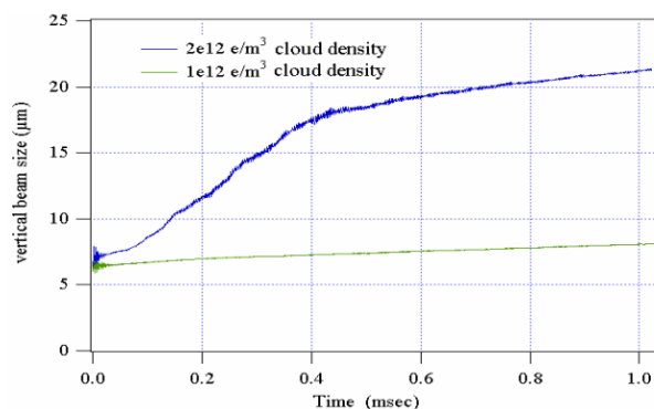
Figure 1: Simulation of single-bunch beam instability from electron cloud in GLC/NLC Damping Ring.
