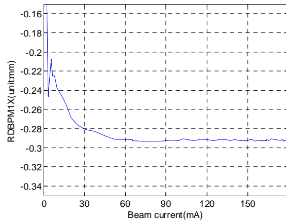
Figure 4: The dynamic range of DBPM.
