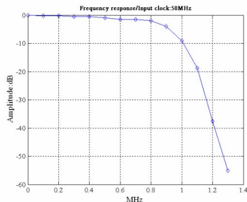
Figure 5: Bandwidth of DBPM system for turn-by-turn mode.
