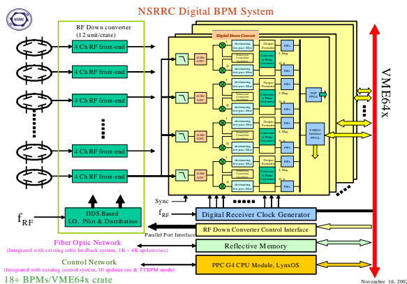
Figure 1: System block diagram of the digital BPM.
