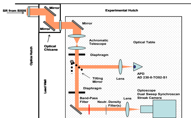
Figure 2: Schematic setup of streak camera and filling pattern measurements on the optical table in the experimental hut of X05DB diagnostic beamline.
