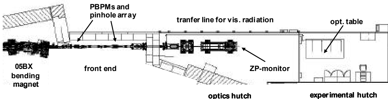
Figure 1 : SLS diagnostic beamline at 05BX bending magnet. The layout shows the generic front end with photon beam position monitors and pinhole array, the optics hutch with the zone plate profile monitor and the experimental hutch with an optical table for experiments with visible synchrotron radiation.
