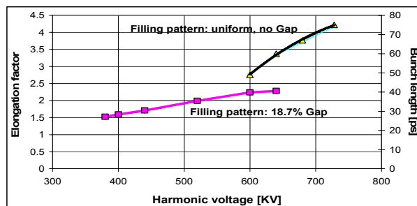
Figure 4: Streak camera measurement, average bunch length in the SLS storage ring with 300 mA uniform filling pattern and with 18.7% empty gap.
