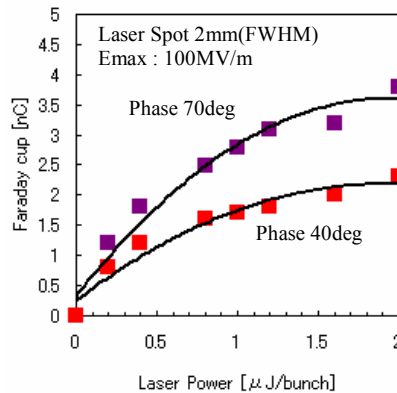
Fig.4: Emitted charge from the RF gun vs. laser power to the cathode with a spot size of 2mm(FWHM).
