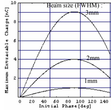
Fig.3: Predictions for the maximum extractable charge vs. the initial phase as the function of the beam size.
