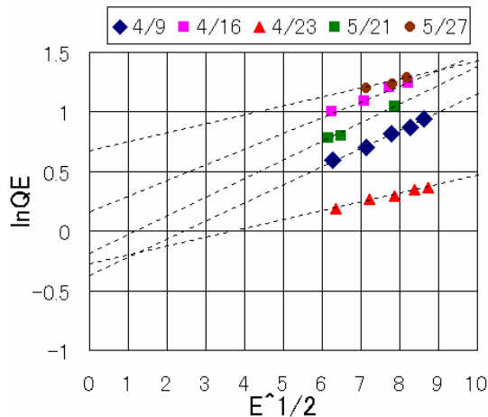
Fig.6: Plot of \ln QE vs. E^{1/2} to estimate the quantum efficiency QE_0 .
