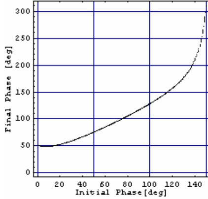
Fig. 1: The final phase vs. the injection phase.
