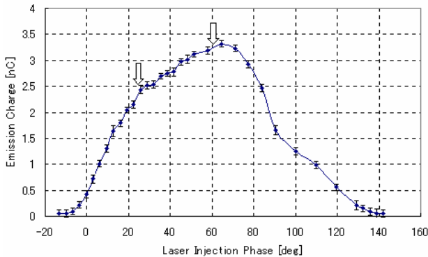
Fig.5: Emission charge vs. laser injection phase at the date of 4/16. Data points between two arrows was used for the Plot of \ln QE vs. E^{1/2} .
