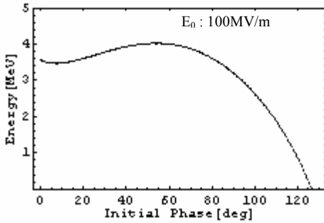
Fig. 2: Output energy at the maximum field of 100MV/m vs. the injection phase.
