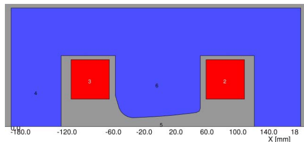
Figure 5. Model of BD magnet
