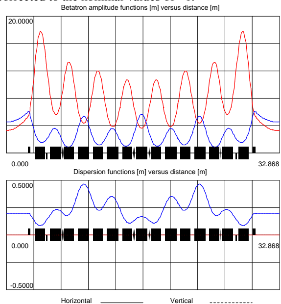
Figure 2. Lattice functions for 1/4 of the ASP Booster. Here also sextupoles are indicated.
