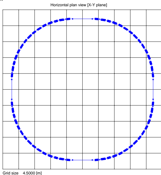
Figure 1. Planar view of booster. Only combined-function and quadrupole magnets are indicated.
