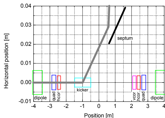
Figure 3. Injection process (electron beam coming in from right)
