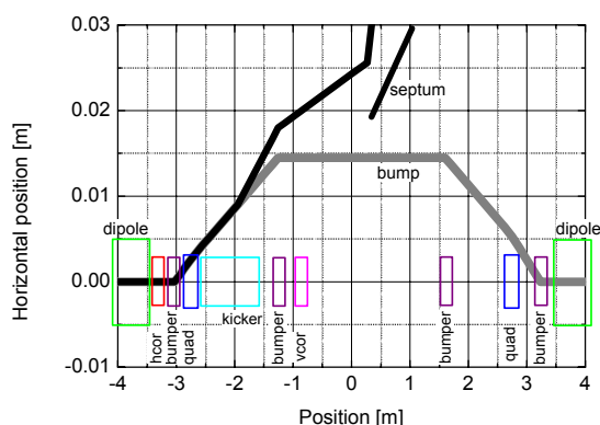
Figure 4. Extraction process (electron beam coming in from left).
