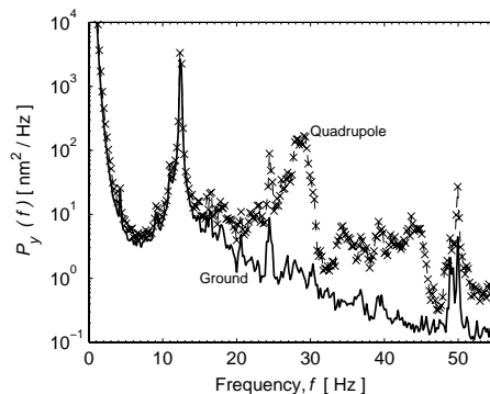
Figure 4: Vertical power spectral density as measured simultaneously on the ground and on a lattice quadrupole.
