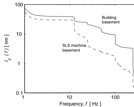
Figure 3: Vertical RMS motions measured after working hours on the floor of the SLS building (solid line) and on the concrete slab where the SLS machine sits (dashed line).
