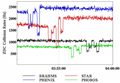
Figure 3: ZDC collision rates from the four experiments as a function of time during an automatic serial optimization.
