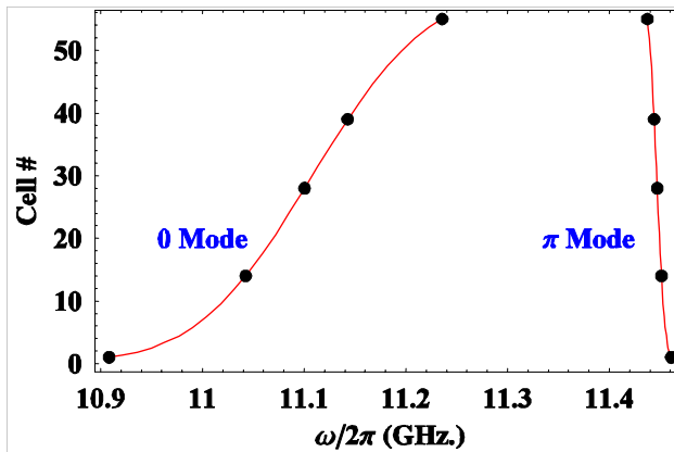
Fig. 3: Cell frequencies for zero and \pi phase advance. The dots are all computed with Omega2P .
