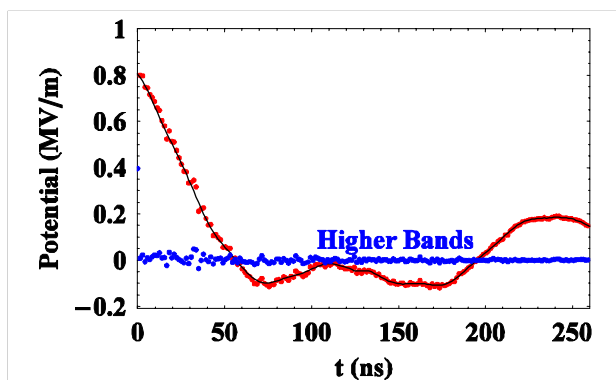
Fig. 2: Longitudinal potential versus time. The potential due to: the complete wake (red dots), first band wake (solid line) and higher order band wake (blue dots).
