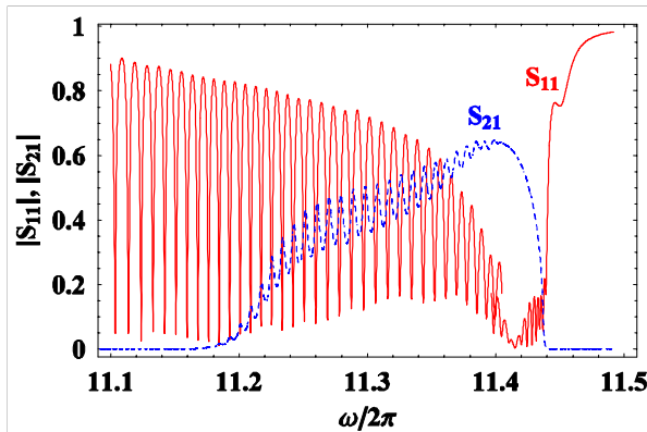
Fig. 4: Input reflection ( S_{11} ) and transmission ( S_{21} ) of accelerating structure.
