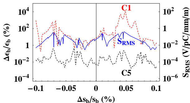
Figure 3: Emittance dilution, \Delta/\epsilon , for a single class of cavities (C1 shown in red) and for five classes of cavities (C5 shown in black). The RMS of the sum wakefield, S_{RMS} , is also illustrated for a single class of cavities (shown in blue).
