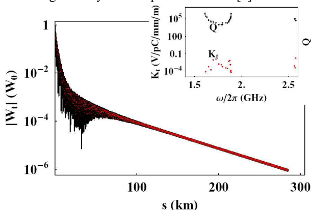
Figure 2: Envelope of TESLA transverse wakefield. The abscissa runs over the distance of the complete bunch train. The ordinate has been normalised with respect to W_0 , (0.11 V/pC/mm/m). The kick factors and Q values are shown in the inset.
