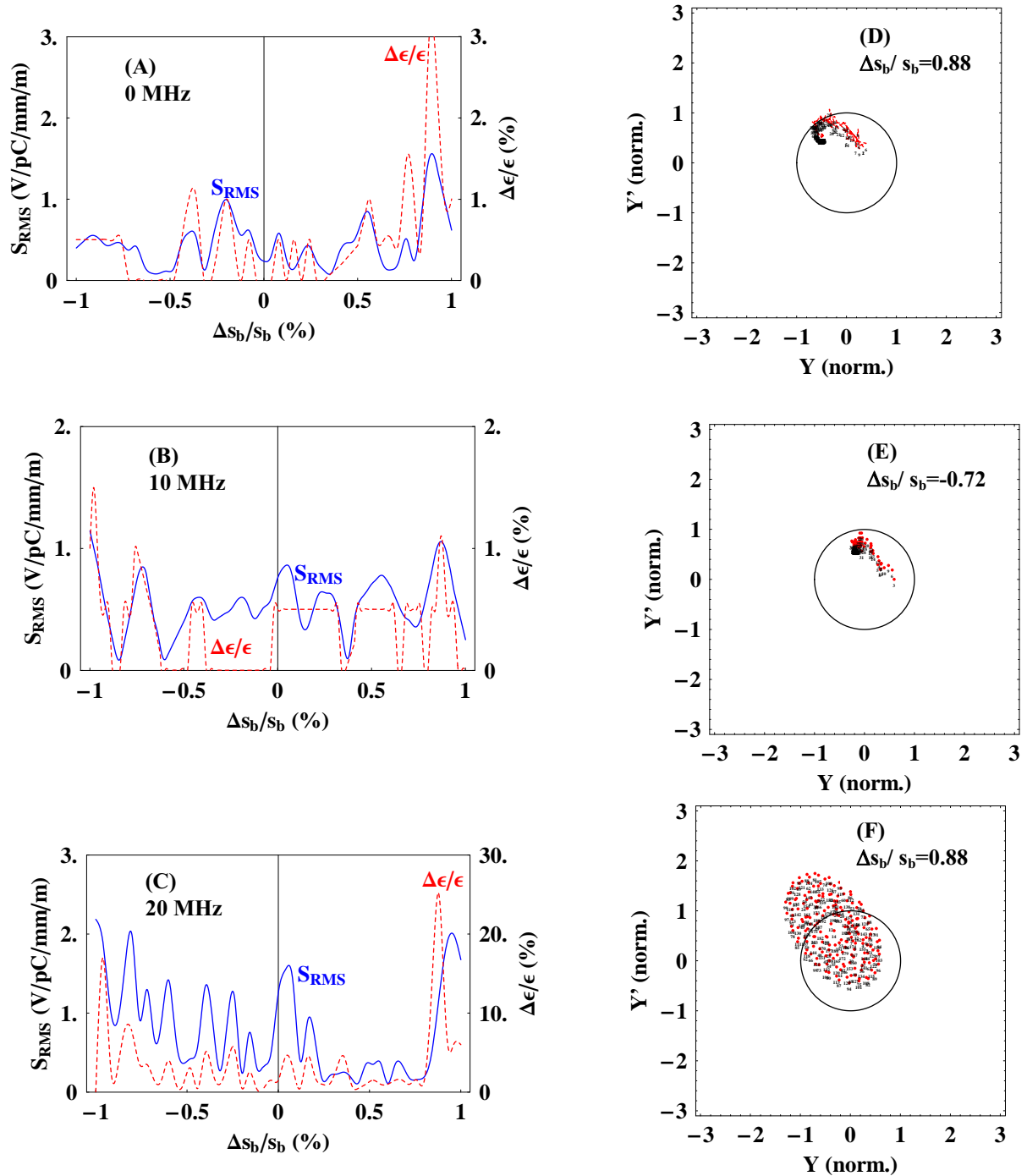
Figure 1: The percentage emittance dilution that occurs at the end of the NLC X-band linac together with the RMS of the random frequency errors is shown in A to C. The abscissa corresponds to a fractional deviation in the bunch spacing expressed as a percentage of the nominal bunch spacing of 42 cm. A small shift in the spacing between bunches leads to a similar effect as would occur from changing all of the cell frequencies by a systematic amount. In all simulations the beam is injected into the linac with an initial offset of 1 \mu\text{m} from the axis of the linac (along the y-axis). The emittance dilution is expressed as a percentage of the injected normalized emittance of 2 \times 10^{-8} m (along the y-axis). Also shown, in D to F, is the normalized phase space at the points of maximum emittance dilution which are given in regions A to C.
