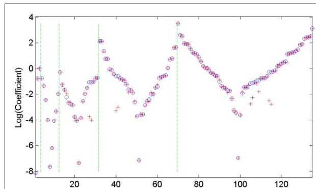
Figure 3: Coefficients in the 5 th order map for x through one period of the BL11 wiggler, calculated with Runge-Kutta integration (blue points), and an explicit symplectic integrator (red crosses). Green lines divide terms of different order.
