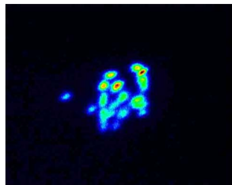
Fig. 5. Result of coherent motion of first 15 turns of the injected beam. The images are superimposed in one frame of CCD
