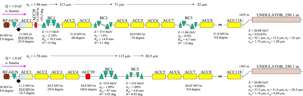
Figure 1: Old (top) and new (bottom) layout for XFEL project. Here all parameters are projected ones.
