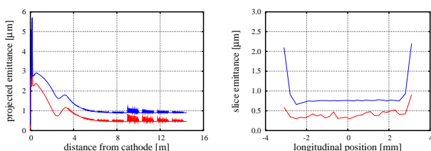
Figure 2: XFEL injector ASTRA simulation results: (left) projected normalized rms emittance up to the end of ACC1, and (right) slice normalized rms emittance at the end of ACC1. Here red (blue) line indicates emittance when rising/falling time is zero (1.5 ps), and thermal emittance is zero ( 0.64 \mu\text{m} ).
