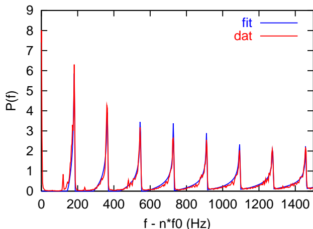
Figure 1: Schottky spectra at injection for Au beams in RHIC and an envelope fit.
