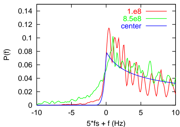
Figure 3: Details of the m = -5 synchrotron sidebands for 1 \times 10^8 and 8.5 \times 10^8 ions. Both have been shifted in frequency and normalized to minimize the chi-square between the data and the blue line referred to as “center”.
