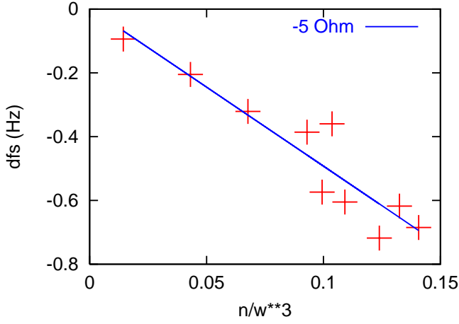
Figure 4: Synchrotron frequency shift versus N/w^3 at injection. N is in units of 10^8 ions and w is in nanoseconds. The crosses mark the data points but don't indicate error bars.
