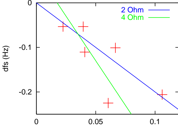
Figure 5: Synchrotron frequency shift versus N/w^3 at store. N is in units of 10^8 ions and w is in nanoseconds. Lines corresponding to \omega_0 L = 2\Omega and \omega_0 L = 4\Omega are shown for reference.
