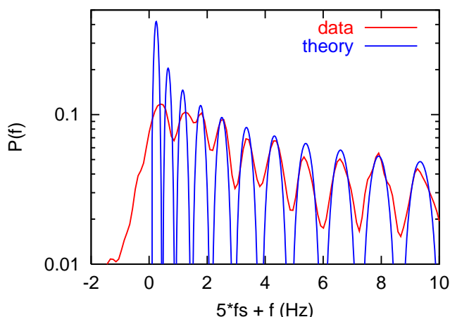
Figure 2: Details of the m = -5 synchrotron sidebands for 1 \times 10^8 ions. The blue line is a fit of equation (9) assuming constant \rho(\tau) .
