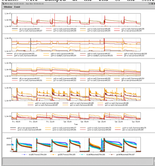
Figure 2. Pressure gauges in five “warm” yellow ring areas are presented for seven gold beam stores.
