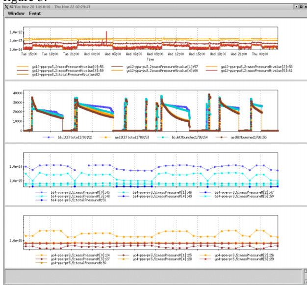
Figure 3. Residual gas analyzers data in three areas of RHIC during the gold-gold run. The largest signals are from the hydrogen molecules.
