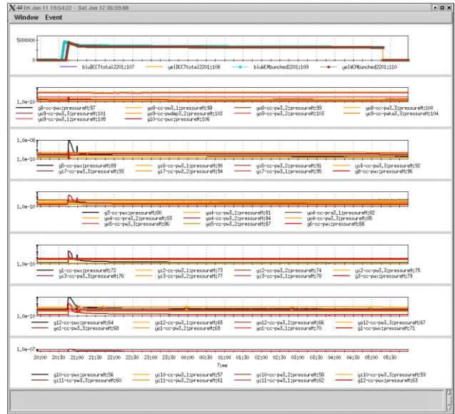
Figure 4. The two proton stored beams are presented at the top of the figure, while the vacuum gauge signals in the yellow “warm” regions follow below.
