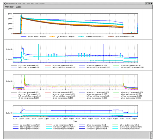
Figure 1. The vacuum signals from three of six warm sectors are shown together with the two “blue” and “yellow” beam signals, during the typical gold store.
