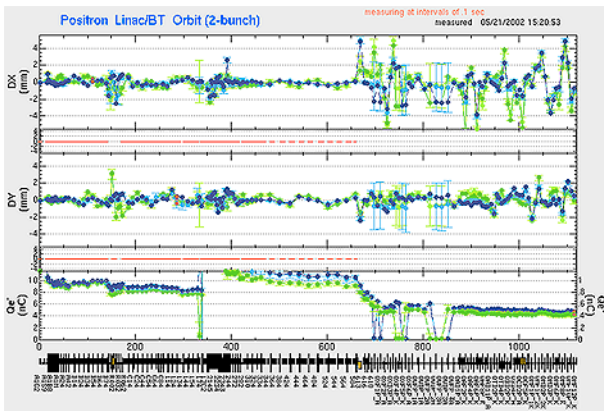
Figure 2: Double-bunch Injection
