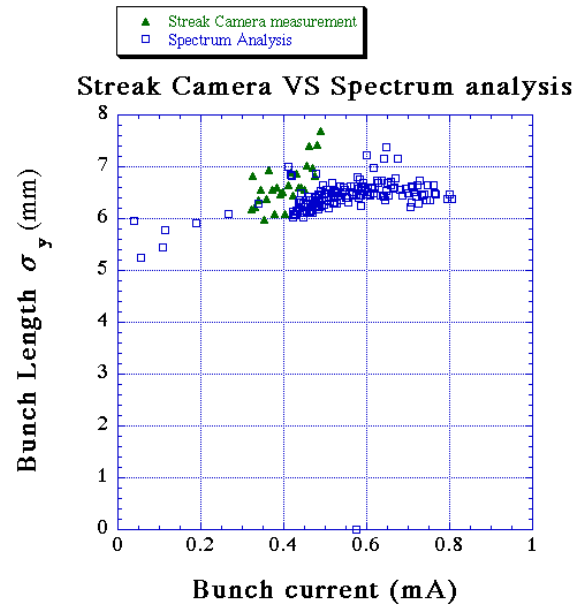
Figure 4: Comparison of the bunch length measurement by the streak camera and by the spectrum analysis
