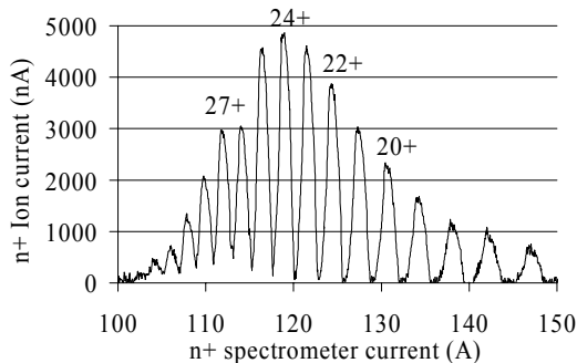
Figure 7: \text{Pb}^{n+} 1+ \rightarrow n+ charge breeding.
