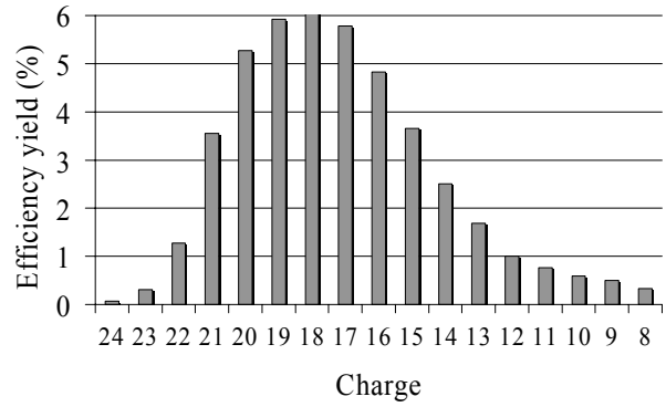
Figure 3: ^{115}\text{In} charge breeding efficiency.
