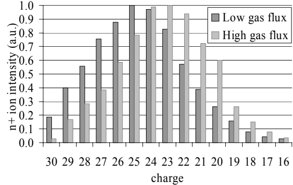
Figure 4: Charge state distribution versus gas flux.
