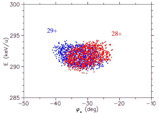
Figure 4: Longitudinal phase space at the end of the 80.5 MHz RFQ with two uranium charge states (28,29).
