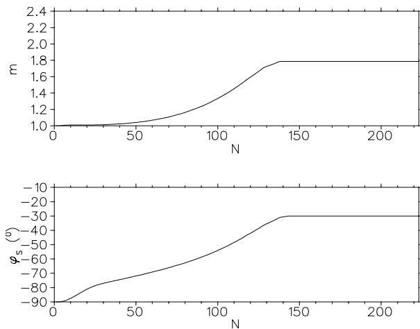
Figure 2: Modulation and synchronous phase of the 80.5 MHz RFQ.
