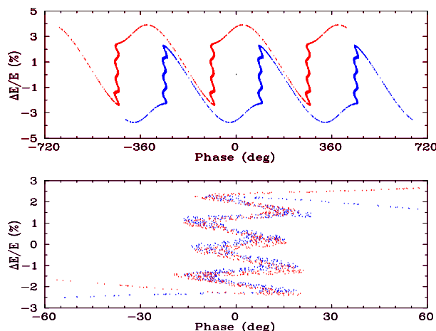
Figure 1: Top: Longitudinal input phase space at the entrance of the RFQ (red=U 29+ , blue=U 28+ ). Bottom: Phase space scaled to the RFQ frequency.
