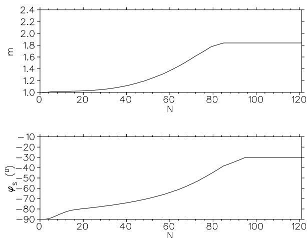
Figure 5: Modulation and synchronous phase of the 57.5 MHz RFQ.
