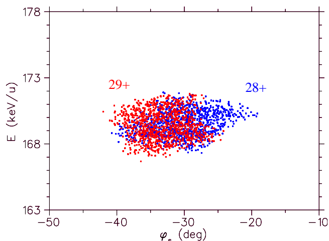
Figure 7: Longitudinal phase space at the end of the 57.5 MHz RFQ with two uranium charge states (28,29).
