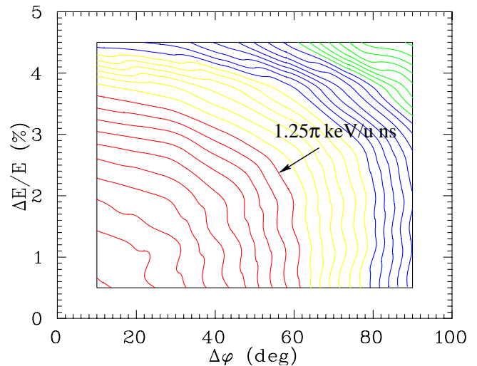
Figure 3: Contour plot of the longitudinal emittance (80.5 MHz) as function of the energy and phase width of the input beam. The beam consists of two uranium charge states (28,29). The acceptable area is plotted in red. In this area the output emittance is smaller than 1.25 \pi \text{keV/n}\cdot\text{ns} (98% particles).
