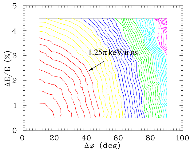
Figure 6: Contour plot of the longitudinal emittance (57.5 MHz) as function of the energy and phase width of the input beam. The beam consists of two uranium charge states (28,29). The acceptable area is plotted in red. In this area the output emittance is smaller than 1.25 \pi keV/u·ns (98% particles)
