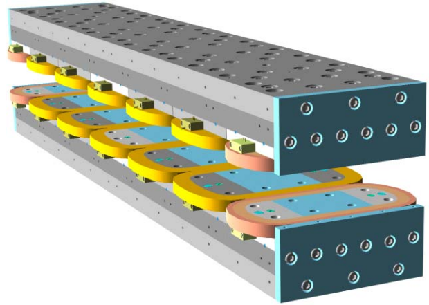
Figure 1: 7 pole superferric wiggler cold mass
