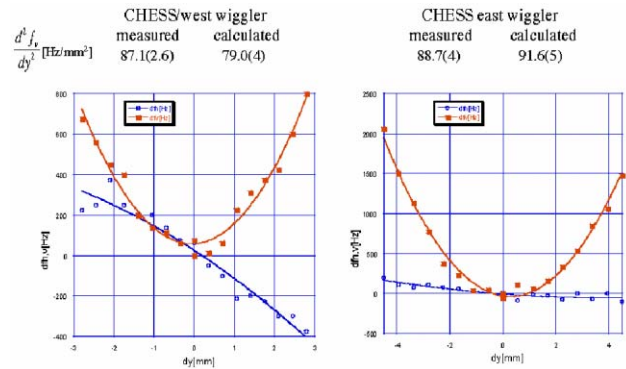
Figure 3 – Measured wiggler cubic terms
