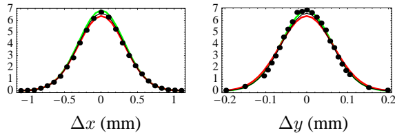
Figure 3: Luminosity scan at H1 after coupling correction. Left: horizontal. Right: vertical. The color code is as in figure 2.
