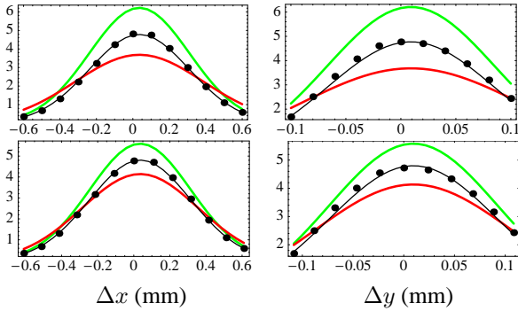
Figure 2: The luminosity scan at H1 for the 72^\circ test optics before the upgrade. Left: horizontal. Right: vertical. The curves show the luminosity data (dots) and a Gaussian fit (black) together with the luminosity (green, upper curve) expected by method a) and the luminosity (red, lower curve) expected by method (b) from the area under the fit. Top: before, Bottom: after taking into account the beam-beam kick and the beam-beam focusing.
