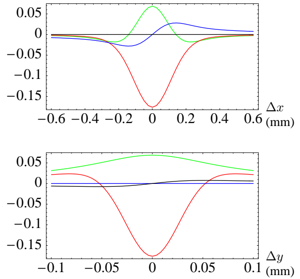
Figure 1: Perturbations due to the beam-beam effect during a luminosity scan in HERA's phase 2. In each figure the central curves describe the beam-beam displacements \delta x (blue) and \delta y (black) in mm. The lowest (red) and the highest (green) curves describe the relative change \delta \beta_y^e / \beta_y^e and \delta \beta_x^e / \beta_x^e of the beta functions respectively.
