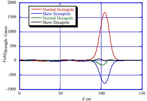
Figure 6: Sextupole and Decapole components
