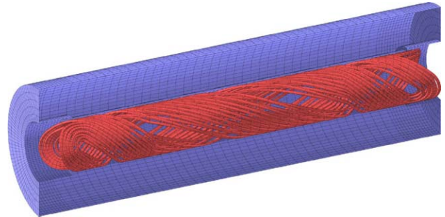
Figure 1: 3D view of the partial helical snake.
