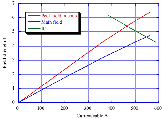
Figure 4: Peak field and IC curve.
