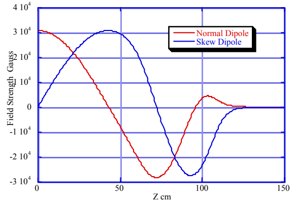
Figure 5: Dipole component.
