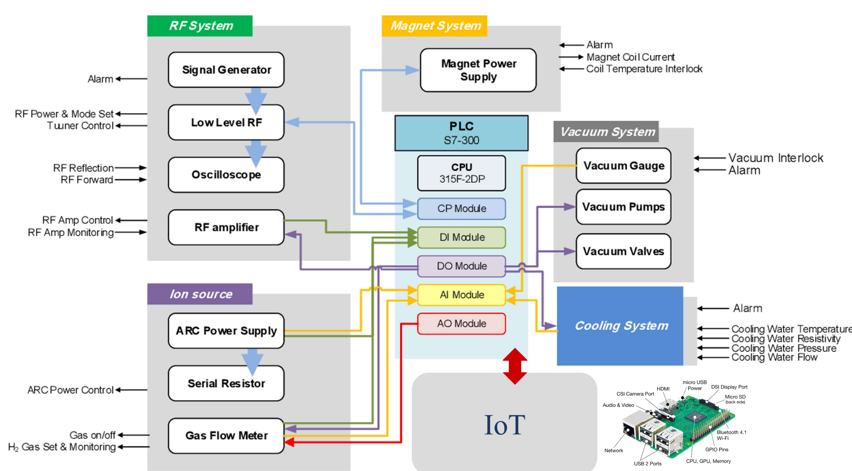
Fig. 1 10 MeV Cyclotron Control System
