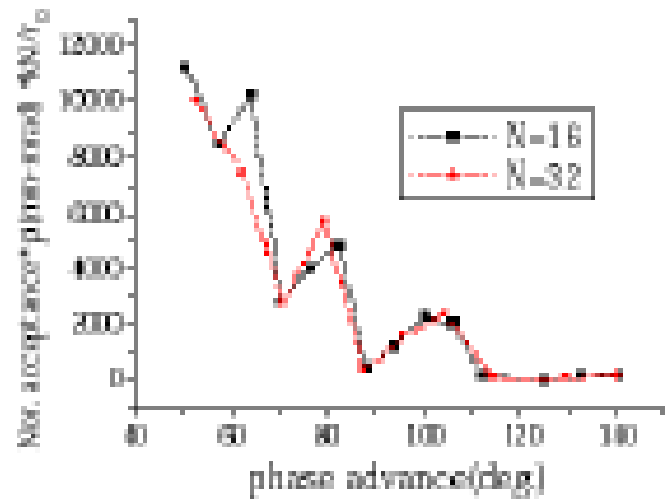
Fig.3 Dynamic apertures
