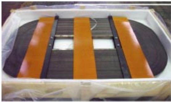
Fig. 4 MA core for rf cavity.
