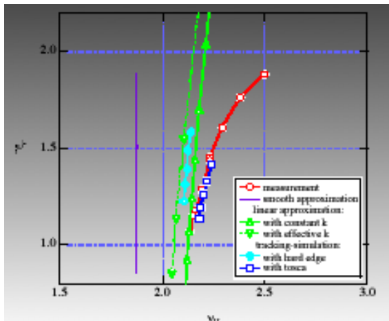
Fig.2 linear, hard edge, tracking
