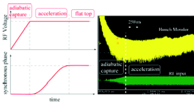
Fig. 8 First beam acceleration.
