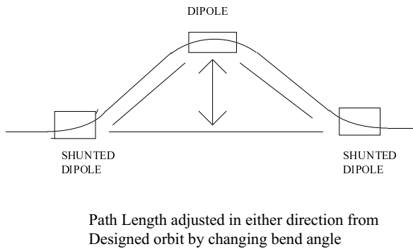
Figure 5 Dogleg System
